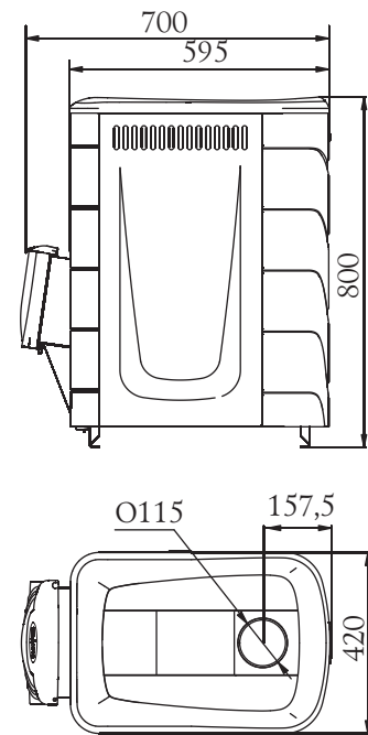
Figure 3. Overall sizes of the stove "Tunguska 2011" cshort of the fuel channel.
