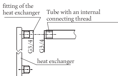
Figure 15. Direct connection of the pipeline
