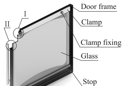
Figure 17. Repair of translucent screen of «Vitra» model door
