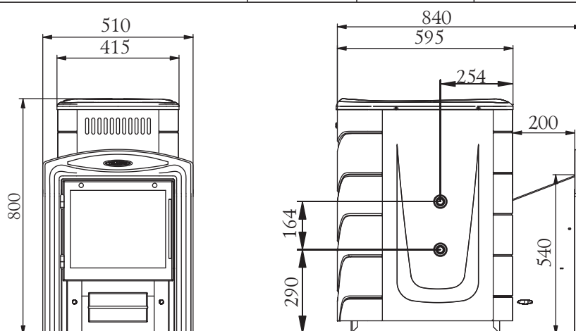
Figure 1. Overall sizes of the stove “Tunguska 2011 Vitra”
