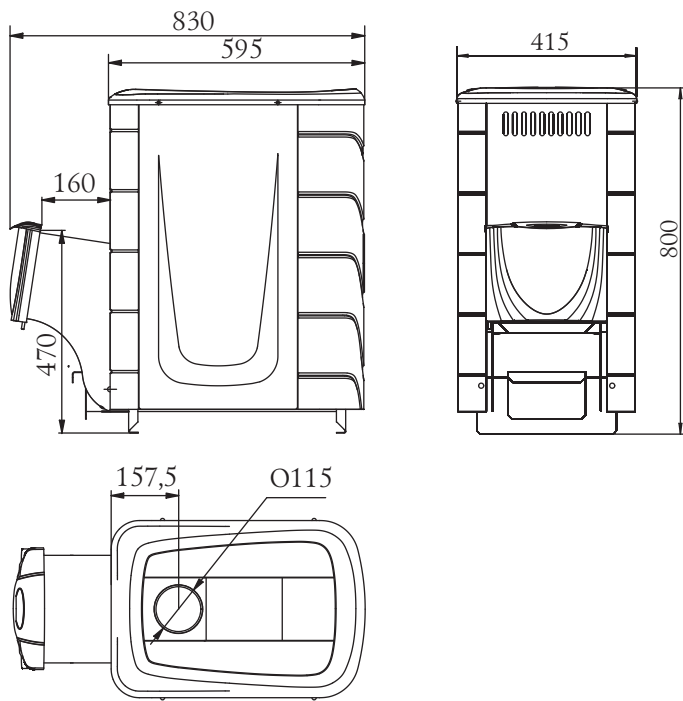
Figure 2. Overall sizes of the stove "Tunguska 2011"
