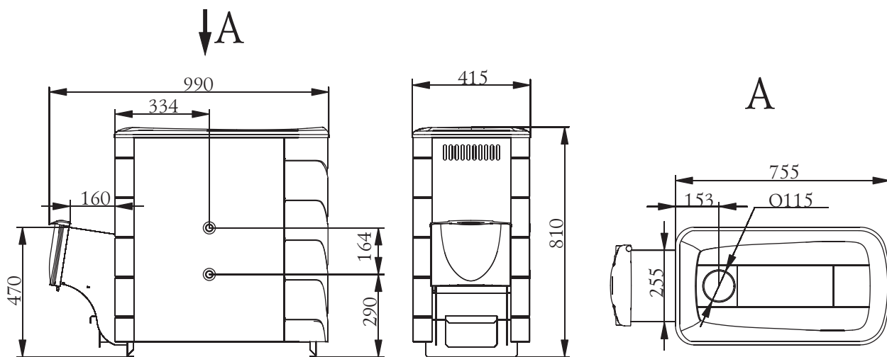
Figure 5. Overall sizes of the stove "Tunguska XXL 2013"
