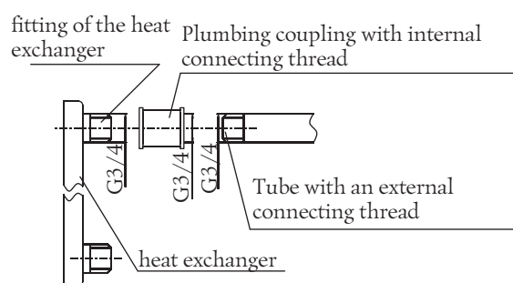
Figure 16. Pipe connection through coupling
